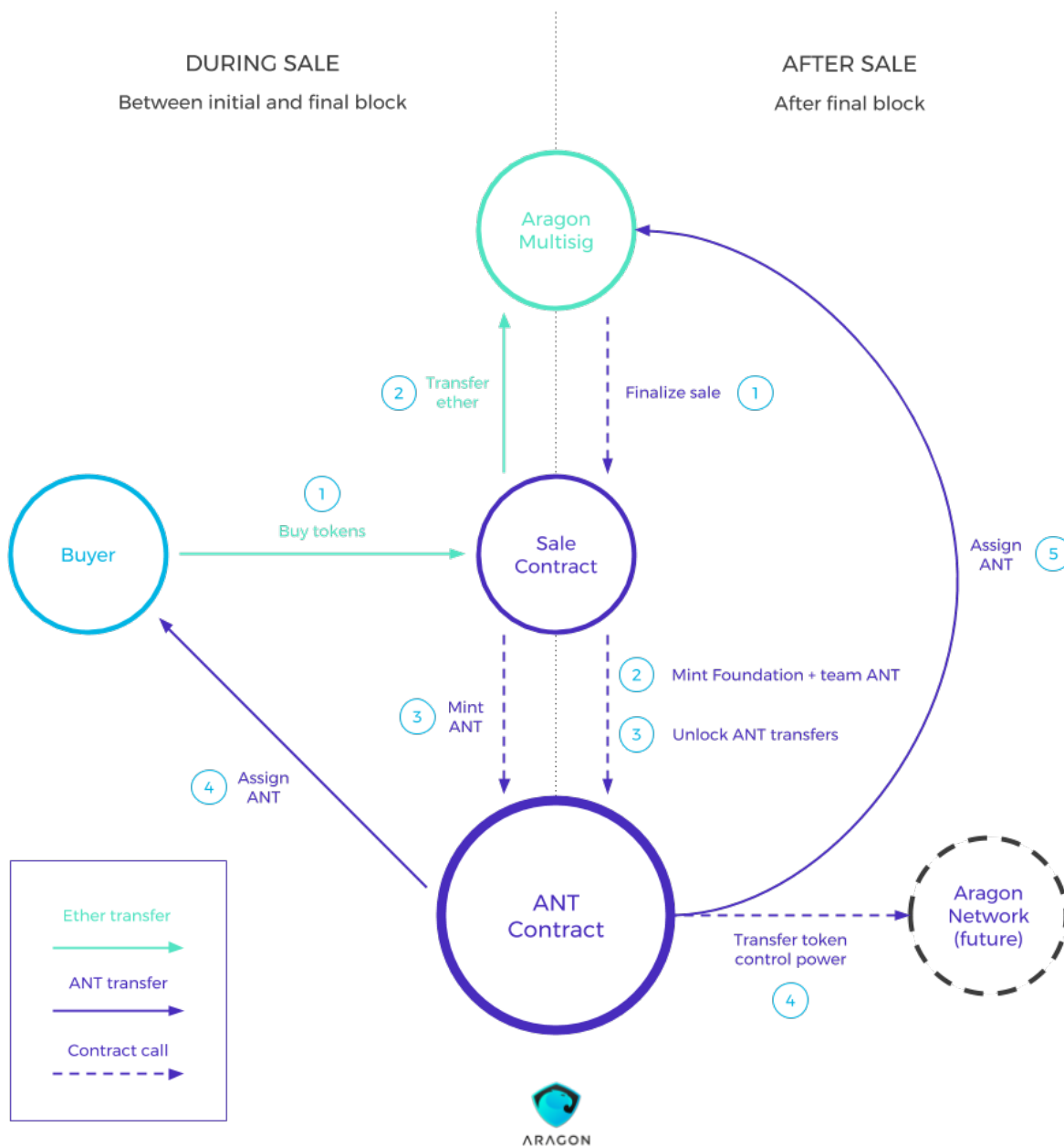
Figure 5.1 B: The Aragon Token Sale mechanism
