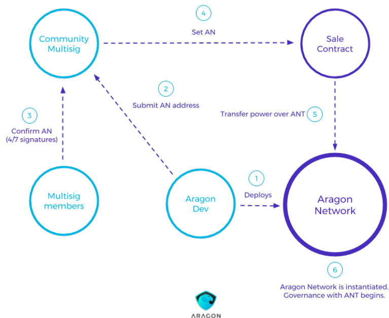
Figure 5.1 A: Aragon Network deployment mechanism
